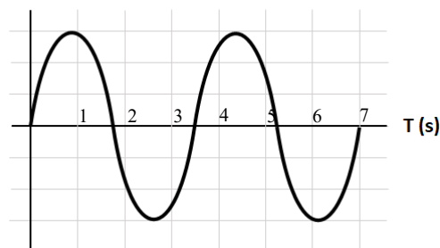
D_x(x = 0, t)
