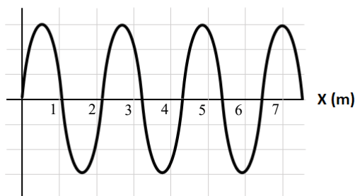
D_x(x, t = 0)
